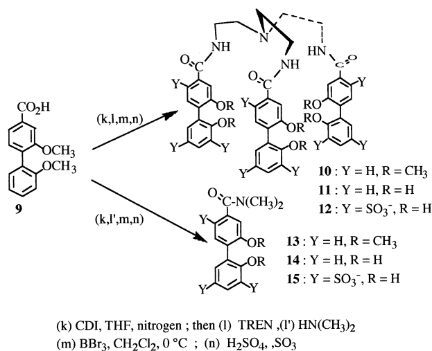
Figure 2. Synthesis of the ligands
