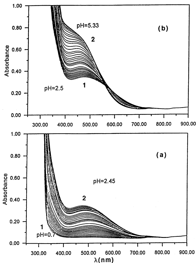
Figure 6. UV/Vis absorption spectra of \text{Fe}^{3+} – L_m ligand as a function of pH; (a) 1: pH = 0.7; 2: pH = 2.45; (b) 1: pH = 2.5; 2: pH = 5.3; [\text{Fe}^{3+}] = [\text{L}_m] = 0.25 \text{ mmol dm}^{-3} ; I = 0.1 \text{ mol dm}^{-3} ( \text{NaClO}_4 )
