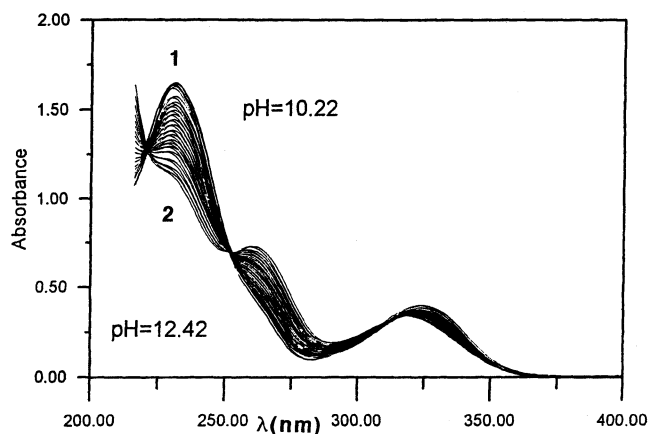
Figure 5. UV/Vis absorption spectra of the L_m ligand as a function of pH; 1: pH = 10.2; 2: pH = 12.4; [L_m] = 0.05 \text{ mmol dm}^{-3} ; I = 0.1 \text{ mol dm}^{-3} ( \text{NaClO}_4 )
