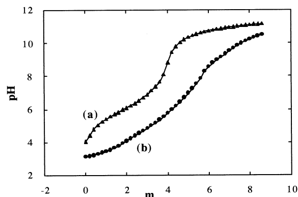
Figure 4. Potentiometric titration curves for (a) 0.5 mmol dm -3 ligand L m ; (b) ligand L m + Fe 3+ 1:1 0.5 mmol dm -3 ; m = moles of base added per mol of ligand; all solutions were at 25 °C and I = 0.1 mol dm -3 (NaClO 4 ); the deprotonation constants of the ligand and the complexation constants were calculated using the SUPERQUAD program [15]
