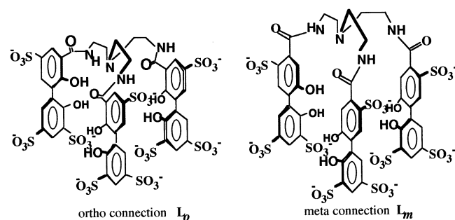
Figure 1. Structural formulae of tris-2,2'-dihydroxybiphenyl ligands
