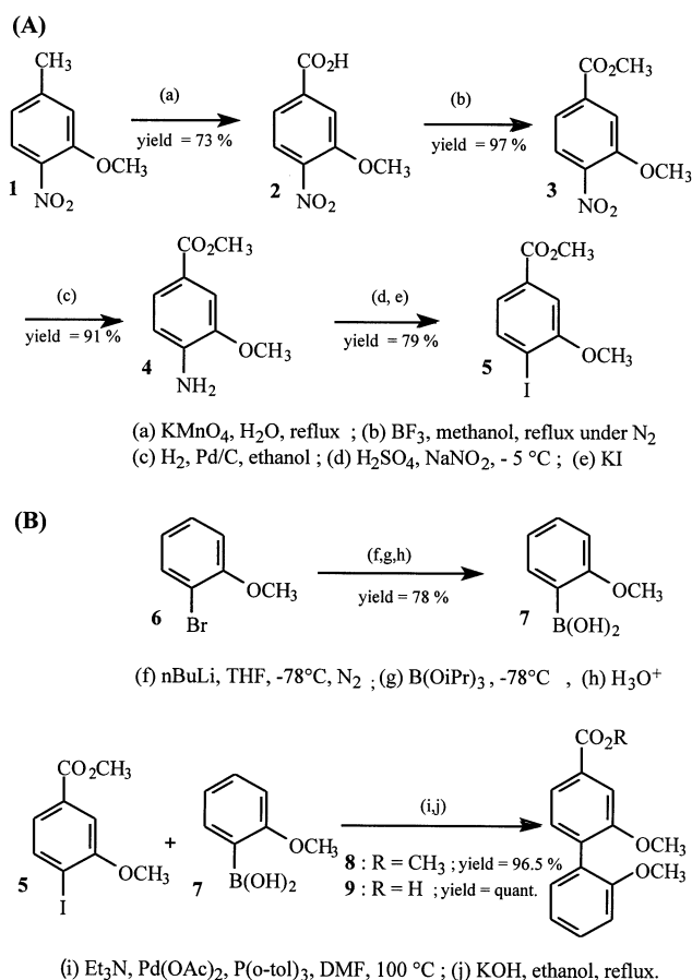
Figure 3. Synthesis of 2,2'-dimethoxy-1,1'-diphenyl-4-carboxylic acid 9
